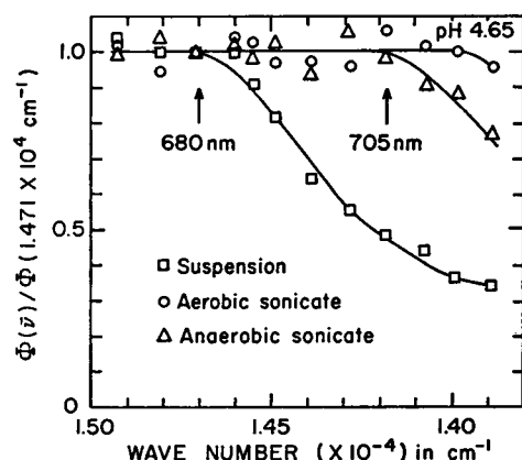
FIGURE 1 Relative quantum yield of fluorescence, \Phi(\bar{\nu})/\Phi(1.471 \times 10^4 \text{ cm}^{-1}) calculated from the excitation and absorption spectra, for a suspension of Chlorella pyrenoidosa and its aerobic and anaerobic sonicates at pH 4.65.
